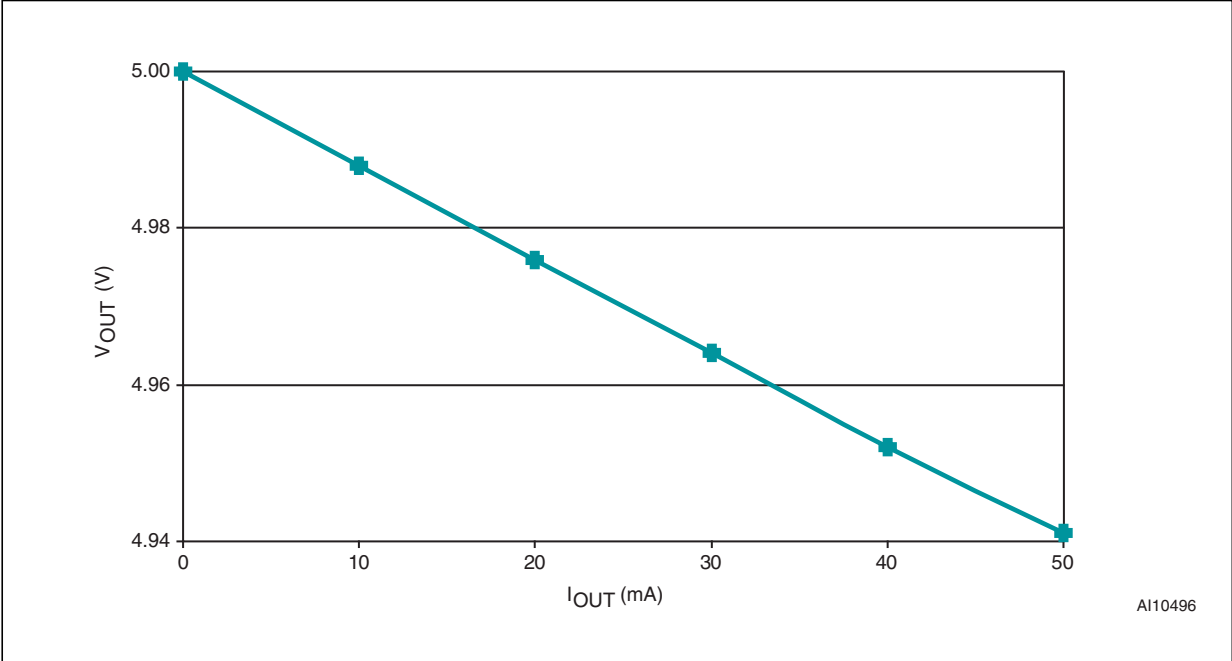
Figure 19. Output voltage vs. load current ( V_{CC} = 5\text{ V} ; T_A = 25\text{ °C} )
