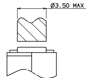
SET MAKER KNOB SIZE (L:3.15mm ONLY)
