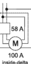
In-line and inside-delta connection of PS S 18/30...300/515
