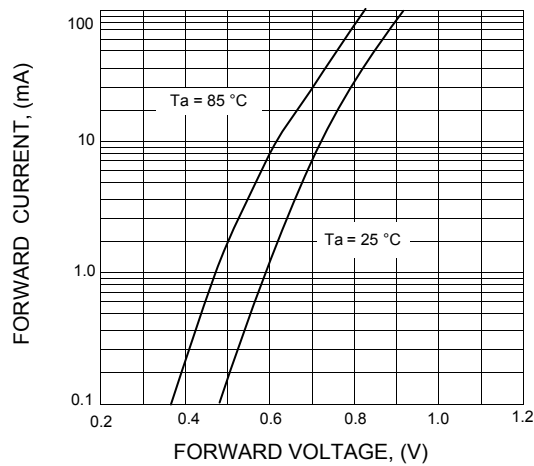
FIG.3 - FORWARD CHARACTERISTICS
