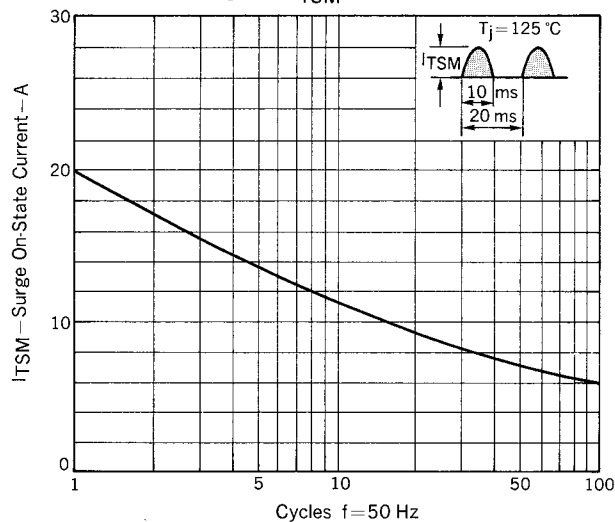
Fig. 10 I_{TSM} RATINGS
