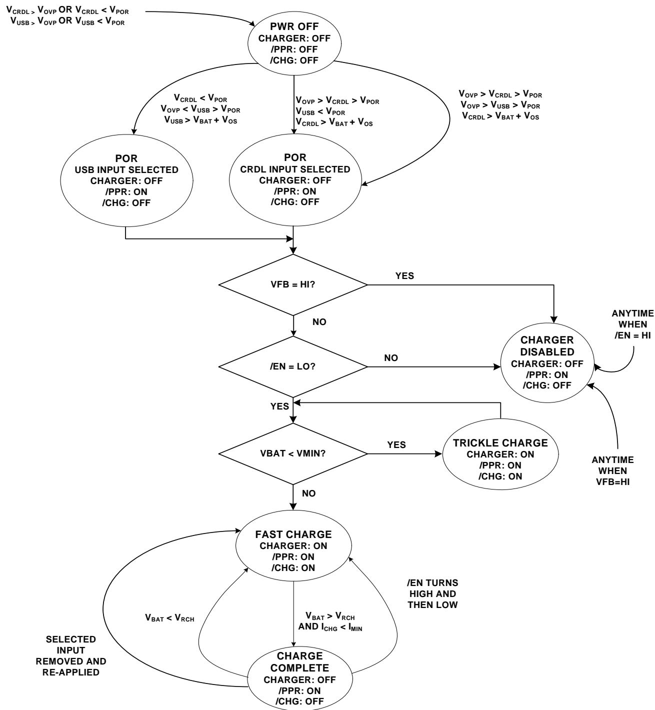
FIGURE 12. STATE DIAGRAM
