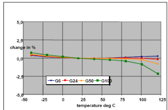
Figure 20: Typical output as function of temperature for all gains
