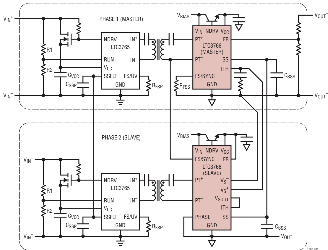
Figure 34. PolyPhase Connections
