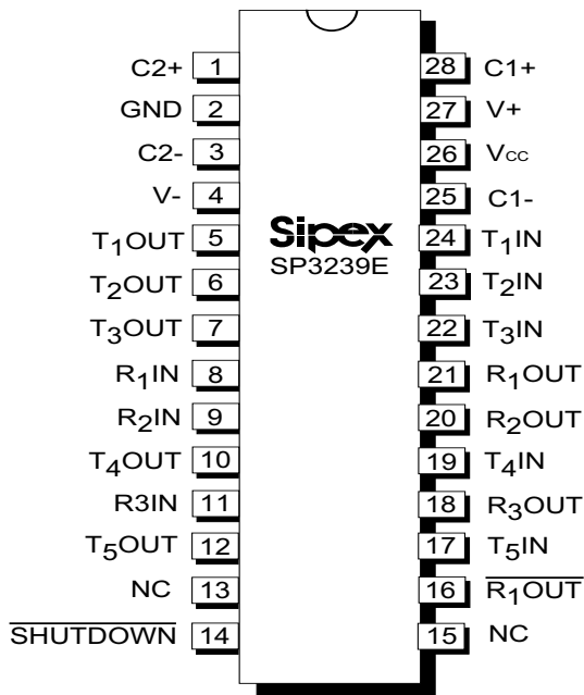
Figure 4. SP3239E Pinout Configuration
