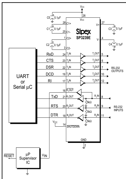
Figure 6. Interface Circuitry Controlled by Microprocessor Supervisory Circuit
