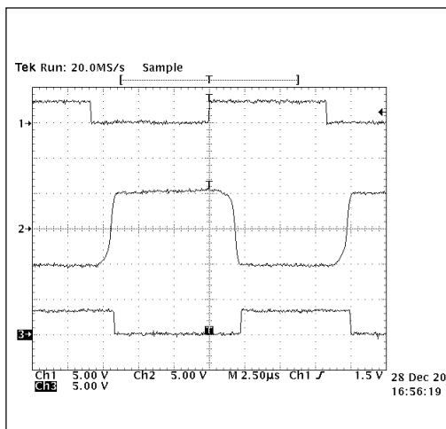
Figure 8. Loopback Test Circuit Result at 120kbps (All Drivers Fully Loaded)
