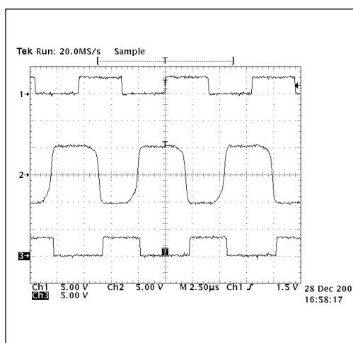
Figure 9. Loopback Test Circuit result at 250kbps (All Drivers Fully Loaded)
