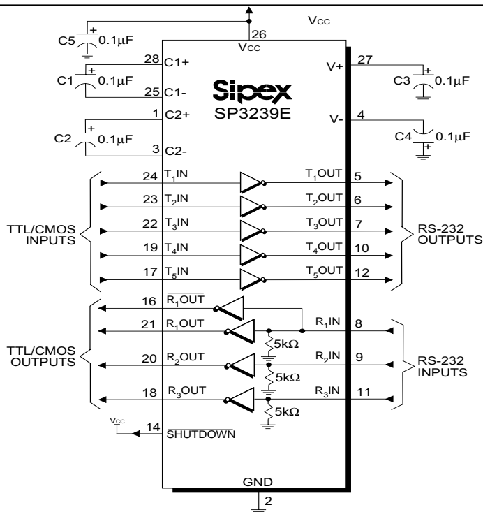
Figure 5. SP3239E Typical Operating Circuit
