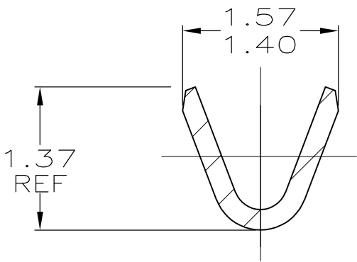
SECTION B-B SCALE 20:1
