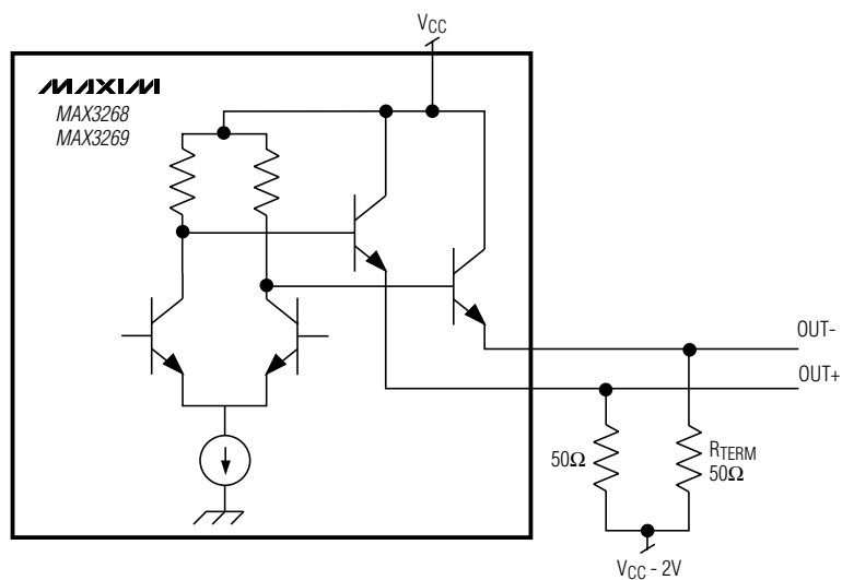
(c) MAX3268/MAX3269 OUTPUT TERMINATION
