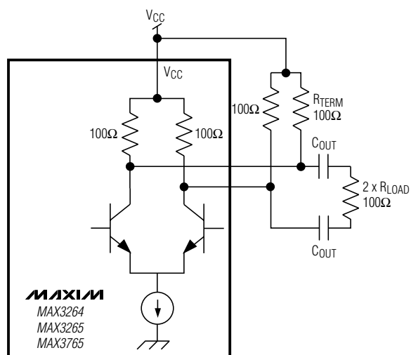
(a) MAX3264/MAX3265/MAX32765 WITH 50Ω TERMINATION
