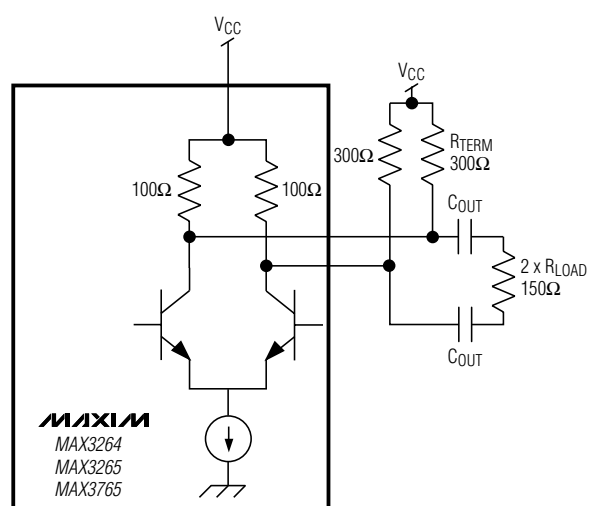
(b) MAX3264/MAX3265/MAX32765 WITH 75Ω TERMINATION
