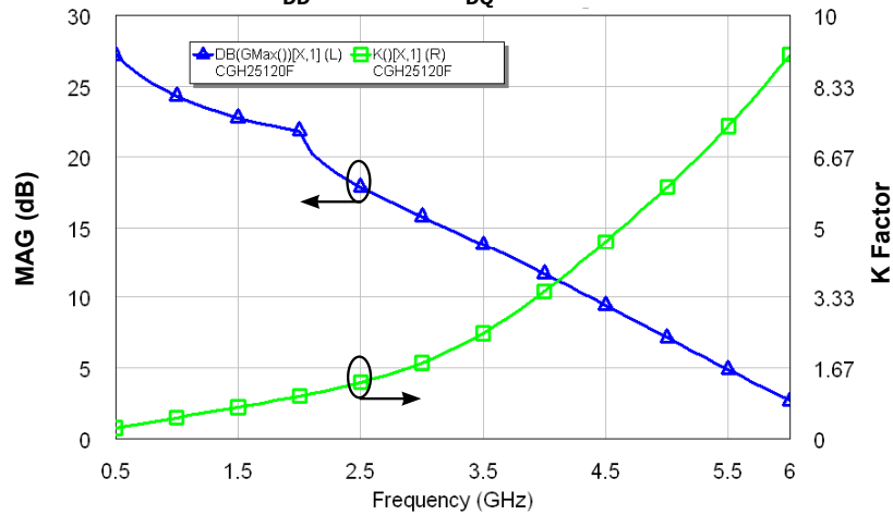
Simulated Maximum Available Gain and K Factor of the CGH25120F V_{DD} = 28 \text{ V} , I_{DQ} = 500 \text{ mA}
