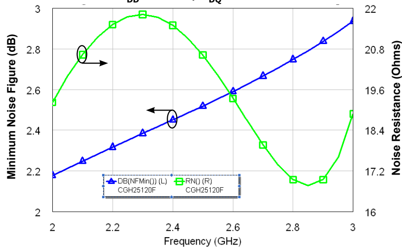
Simulated Minimum Noise Figure and Noise Resistance vs Frequency of the CGH25120F V_{DD} = 28 \text{ V} , I_{DQ} = 500 \text{ mA}
