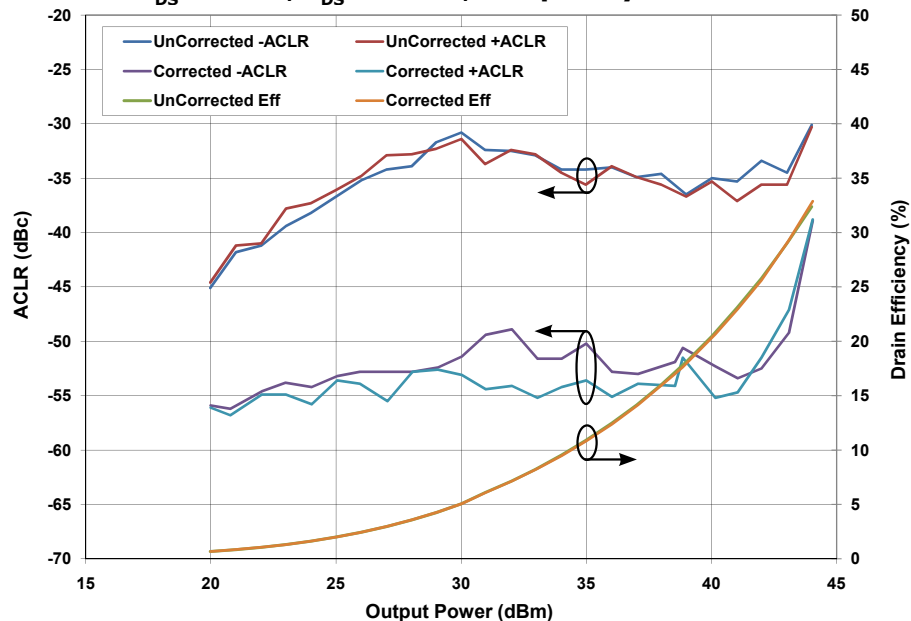
WiMAX Characteristics with and without DPD Correction ACLR and Drain Efficiency vs Output Power of the CGH25120F measured in CGH25120F-TB Amplifier Circuit. V_{DS} = 28 \text{ V} , I_{DS} = 0.5 \text{ A} , Frequency = 2.5 GHz
