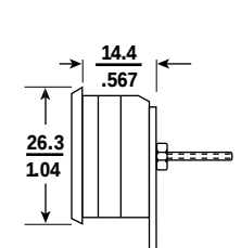
Backlit Bezel Mount Side View
