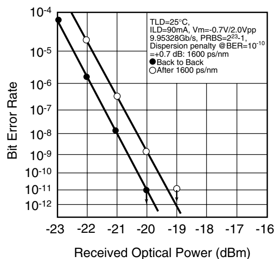
Fig. 6 Transmission Characteristics
