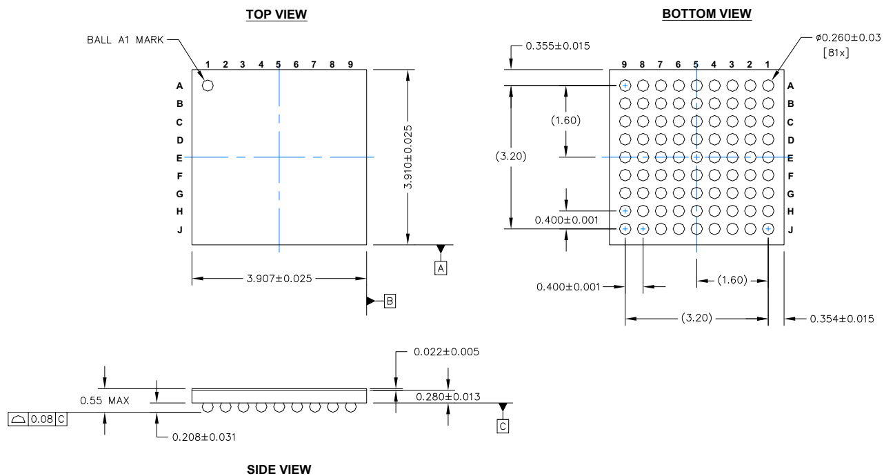
Figure 64. Astoria WLCSP (3.91 × 3.91 × 0.55 mm) FN81B Package Outline, 001-45618
