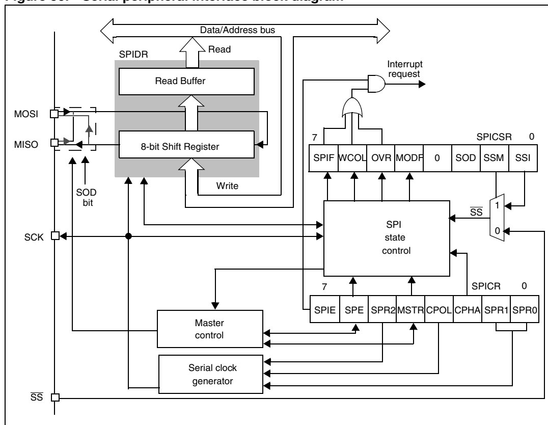
Figure 50. Serial peripheral interface block diagram
