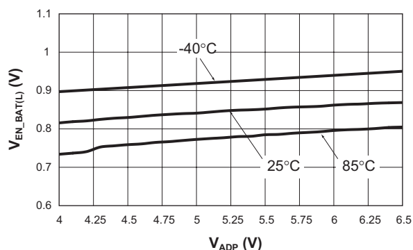
Enable Input Low Voltage vs. Adapter Voltage ( R_{SET} = 8.06k\Omega )
