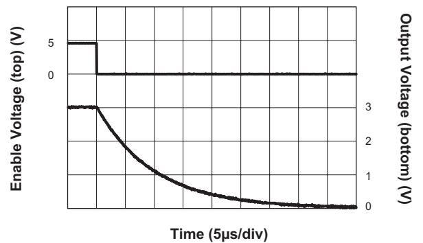
LDO Turn-Off Response Time ( I_{OUT} = 100\text{mA} )
