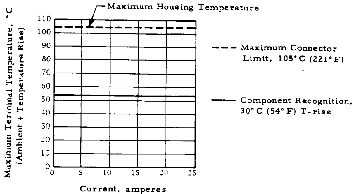
Terminal Temperature vs Current/Circuit, 10 Circuit Housing
