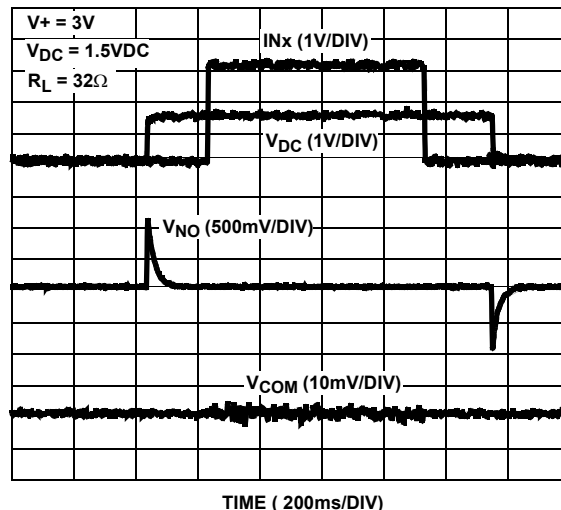
FIGURE 26. CLICK AND POP ELIMINATION 32Ω LOAD 200ms DELAY
