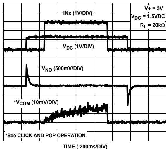
FIGURE 25. CLICK AND POP ELIMINATION 20kΩ LOAD 200ms DELAY
