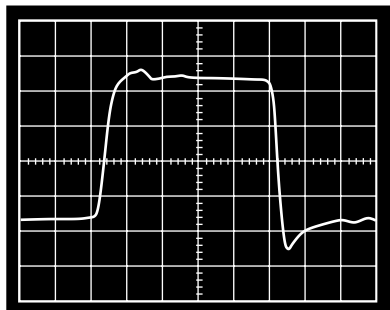
Figure 19. Large Signal Step Response; V_S = \pm 5\text{ V} , V_O = 4\text{ V Step}
