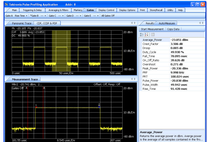
Figure 2 – Pulse profiling software enables a thorough analysis of pulse characteristics.
