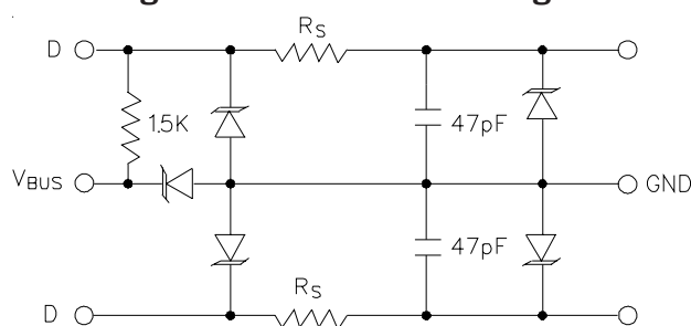
Figure 1 - STF202 Circuit Diagram
