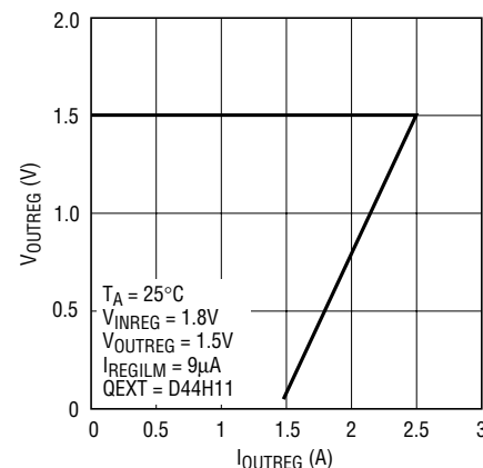
V OUTREG vs Load Current
