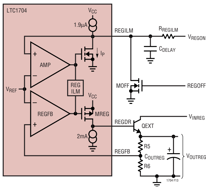
Figure 13. Linear Regulator
