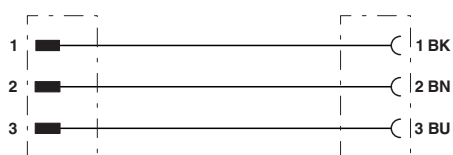
Contact assignment of 7/8" plugs/sockets
