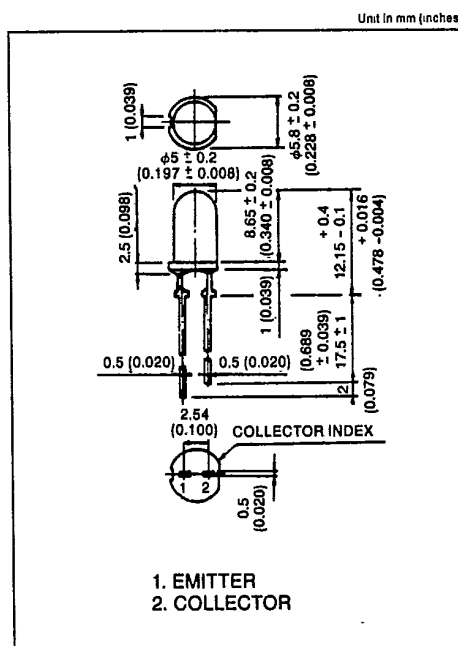
PIN CONNECTION
