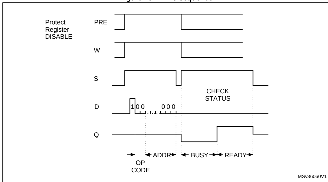
Figure 13: PRDS sequence
