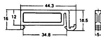
PFP-S Spacer
