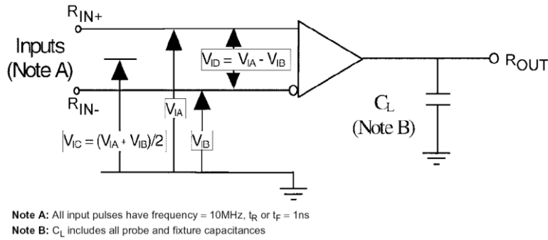
Figure 1. Differential Receiver Voltage Definitions and Propagation Delay and Transition Time Test Circuit
