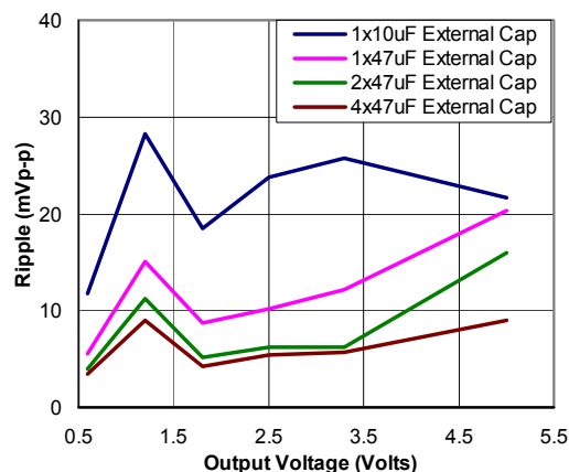
Figure 41. Output ripple voltage for various output voltages with external 1x10 µF, 1x47 µF, 2x47 µF or 4x47 µF ceramic capacitors at the output (20A load). Input voltage is 12V.
