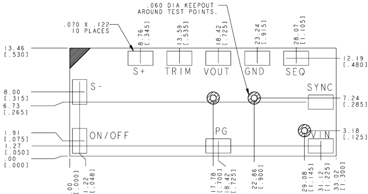
RECOMMENDED FOOTPRINT - THRU THE BOARD -
