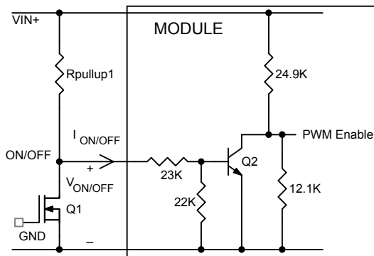
Figure 43. Circuit configuration for using negative On/Off logic.
