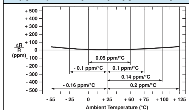
FIGURE 5 - TYPICAL TCR CURVE Z-FOIL
