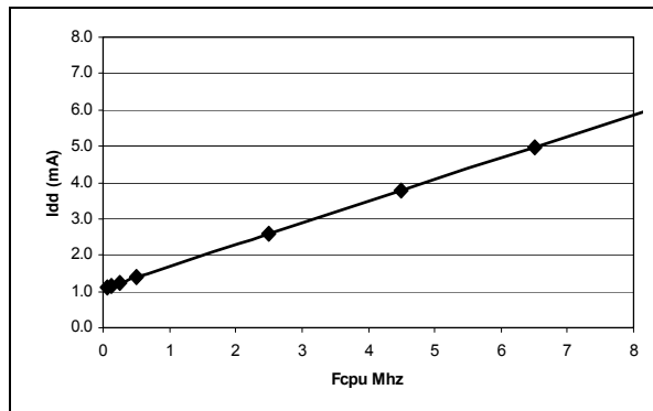
Figure 133. Typical I_{DD} in Wait vs. f_{CPU}
