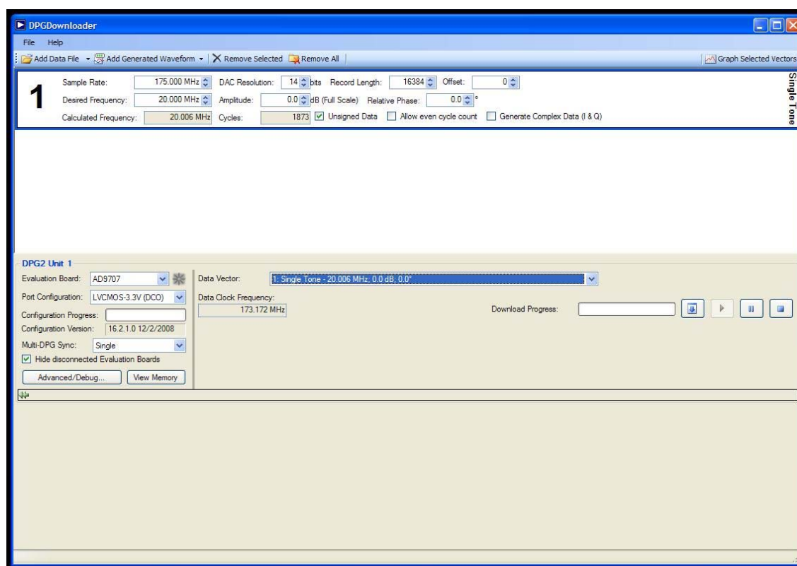
Figure 4: DPG GUI
