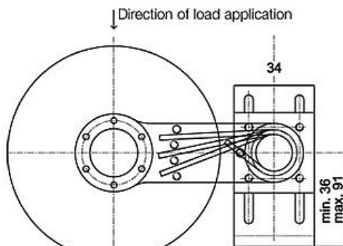
Spring lever, cross section
