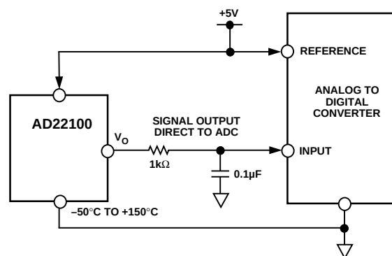
Figure 1. Application Circuit
