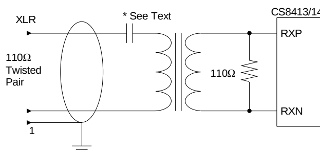
Figure 21. Professional Input Circuit
