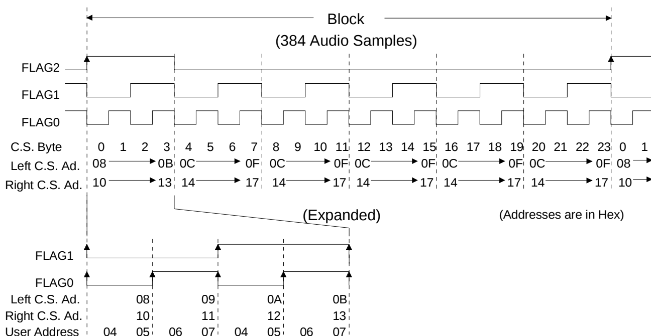
Figure 14. CS8413 Buffer Memory Write Sequence - MODE 2
