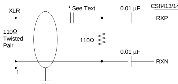
Figure 22. Transformerless Professional Circuit
