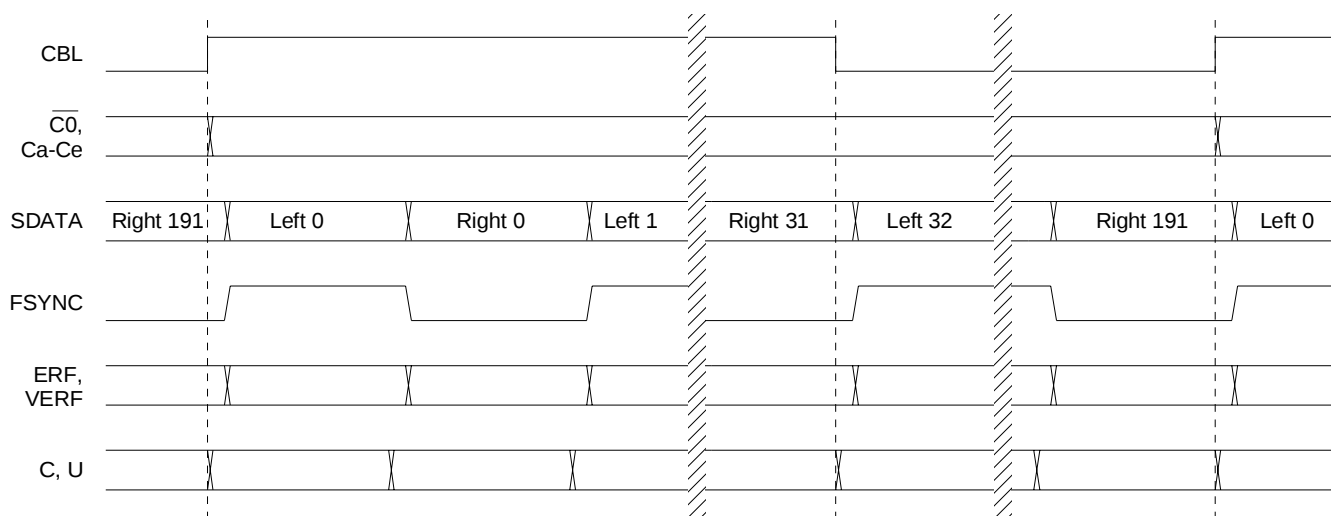
Figure 19. CBL Timing
