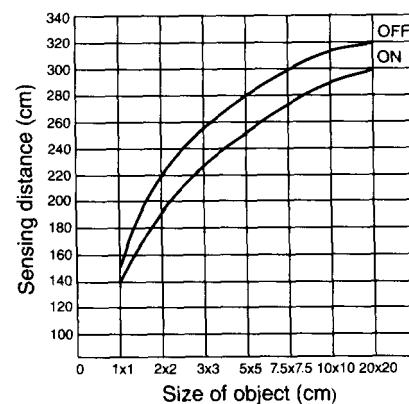
Sensing Distance vs. Set Distance E3S-BT□11
