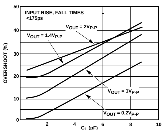
FIGURE 27. MUX2: PULSE OVERSHOOT vs V_{OUT} , C_L ; R_L = 150\Omega
