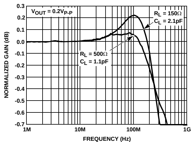
FIGURE 10. MUX2: 0.1dB GAIN FLATNESS
