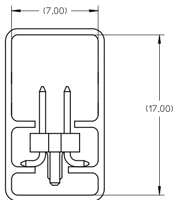
PART IN TUBE ORIENTATION
