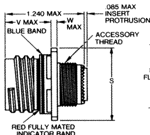
SQUARE FLANGE RECEPTACLE
