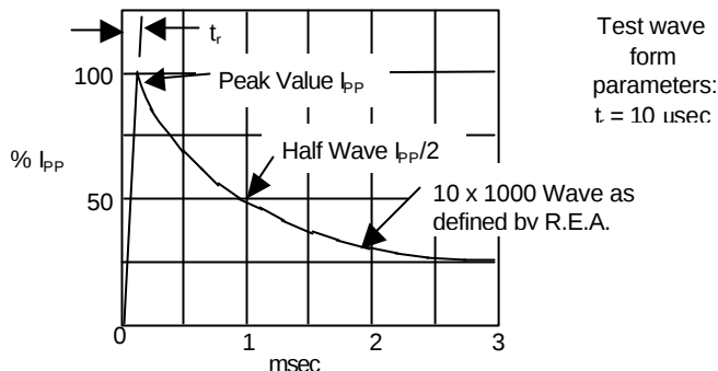
Peak Pulse Current ( \% I_{PP} ) - Versus - Time (t)
