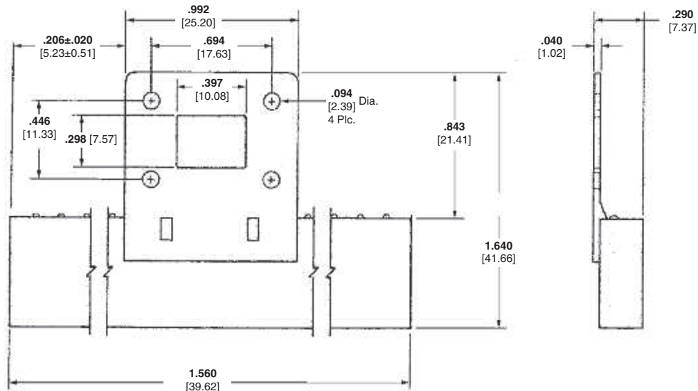
10 Position Receptacle Housing, Part No. 1-102090-0
