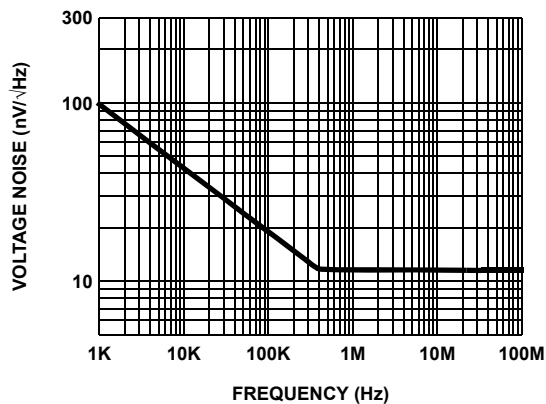
FIGURE 5. INPUT VOLTAGE NOISE SPECTRAL DENSITY vs FREQUENCY
