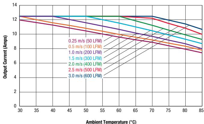
Maximum Current Temperature Derating at sea level (V_{IN}=48V, \text{longitudinal airflow, from } V_{IN} \text{ to } V_{out}, \text{ with baseplate})
