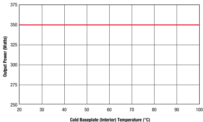
Output Power Derating in Conduction Cooling (Cold Baseplate) Applications (V_{IN}=48V, \text{Ambient Temperature} < 70^{\circ}C)
