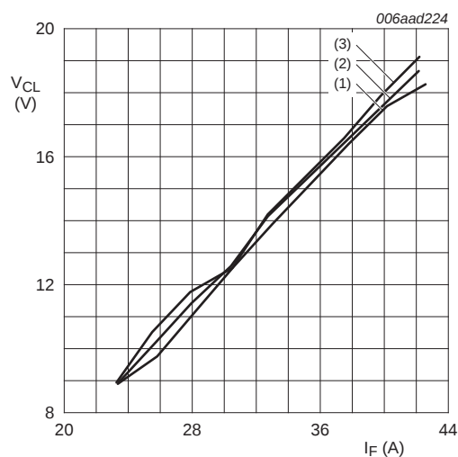
Fig 8. IP4085CX4: peak clamping voltage as a function of forward current
