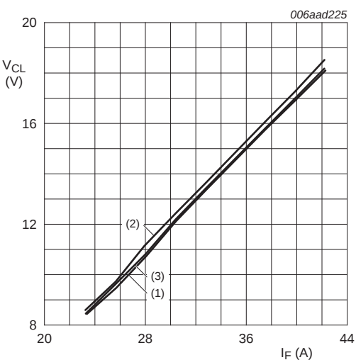
Fig 9. IP4385CX4: peak clamping voltage as a function of forward current
