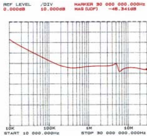
Figure 2: Typical differential-mode insertion loss in a 50Ω circuit
