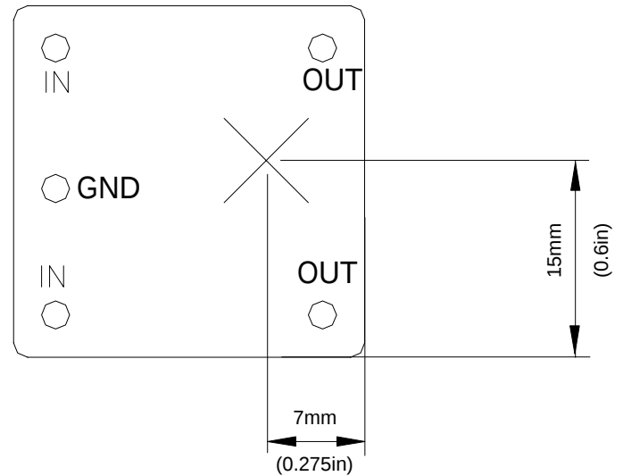
Figure 5: Temperature measurement location
