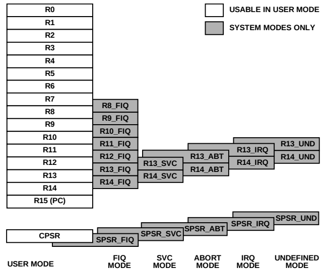
Figure 4. Register Organization
