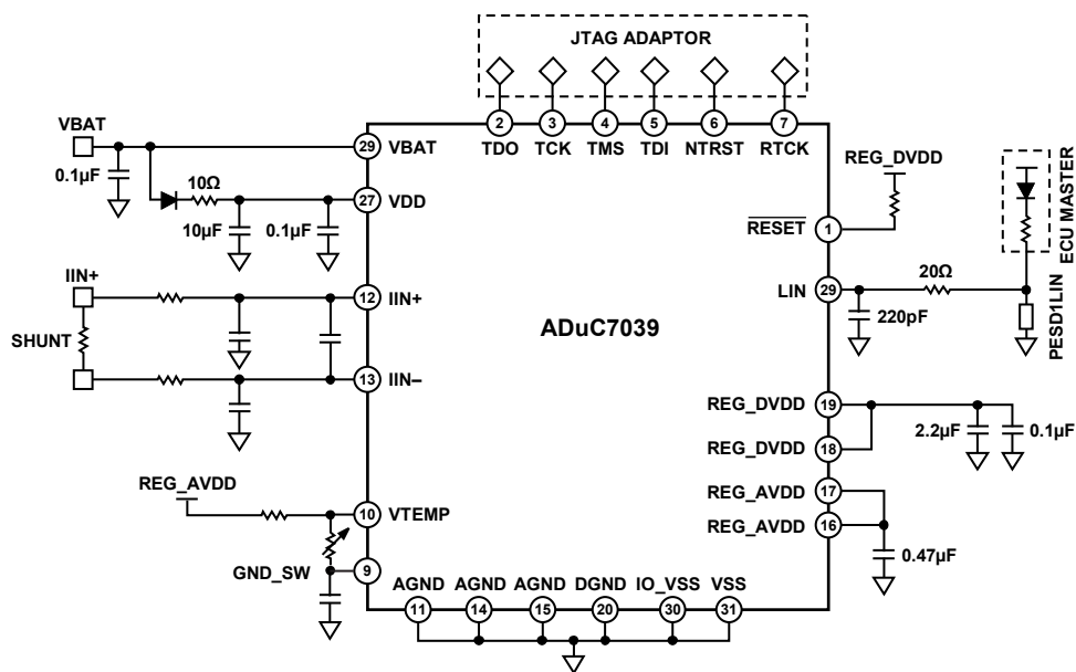
Figure 33. Recommended Schematic
