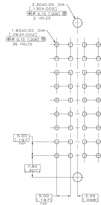
RECOMMENDED PC BOARD LAYOUT
