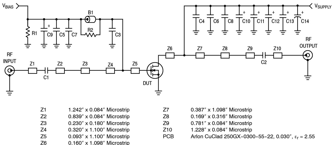
Figure 1. MRF6S19120HR3(SR3) Test Circuit Schematic
