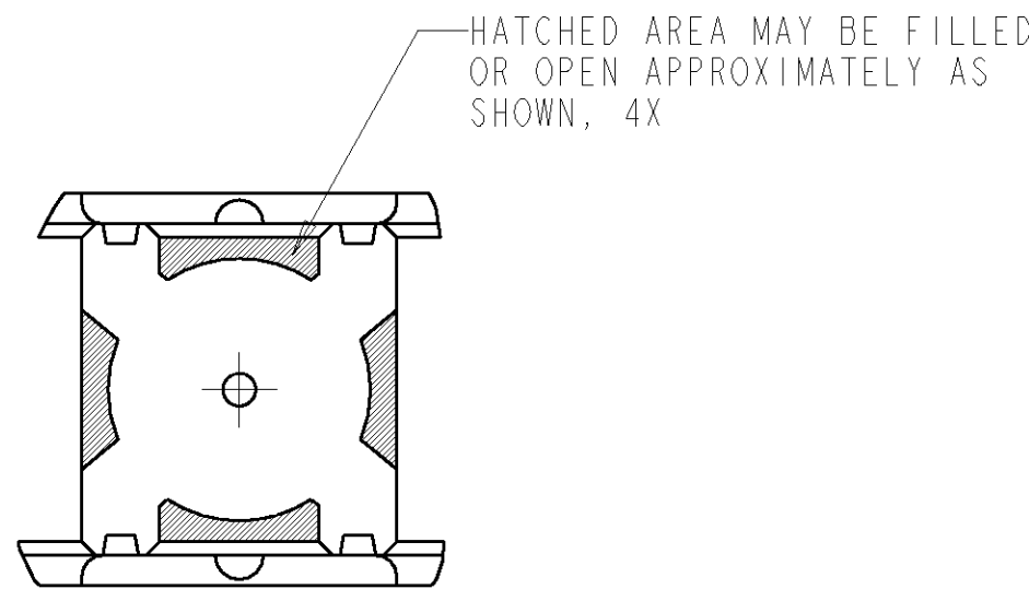
DETAIL A ALTERNATE CENTER BRACE CONFIGURATION
