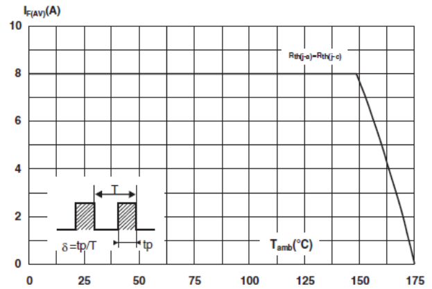
Figure 2. Average forward current versus ambient temperature (δ = 0.5)
